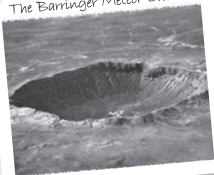
The Barringer Meteor Crater
